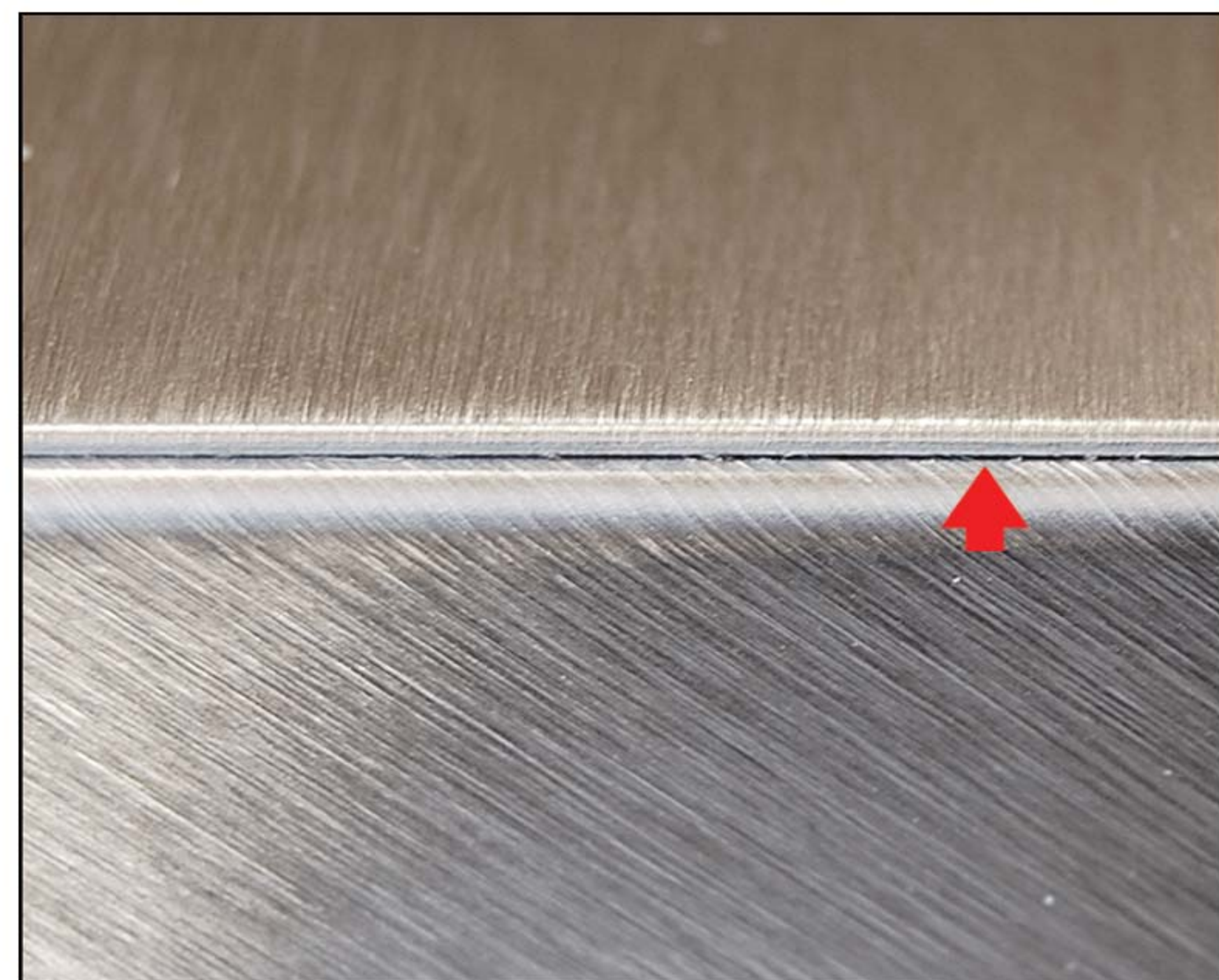
Imperfect Welding Rough Surface
